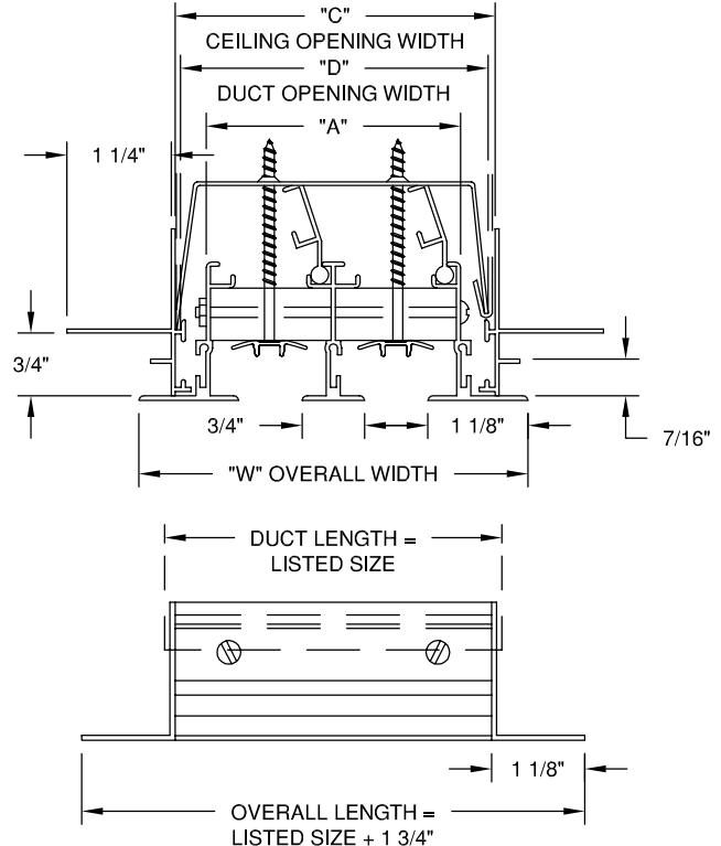
MODEL - 9475-640 w/806 AUXILIARY FRAME
