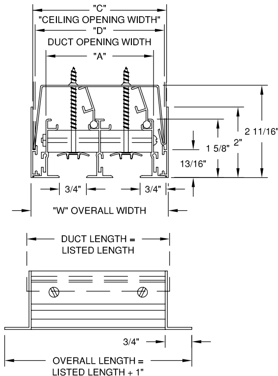
MODEL - 9475-672 w/805 AUXILIARY FRAME
